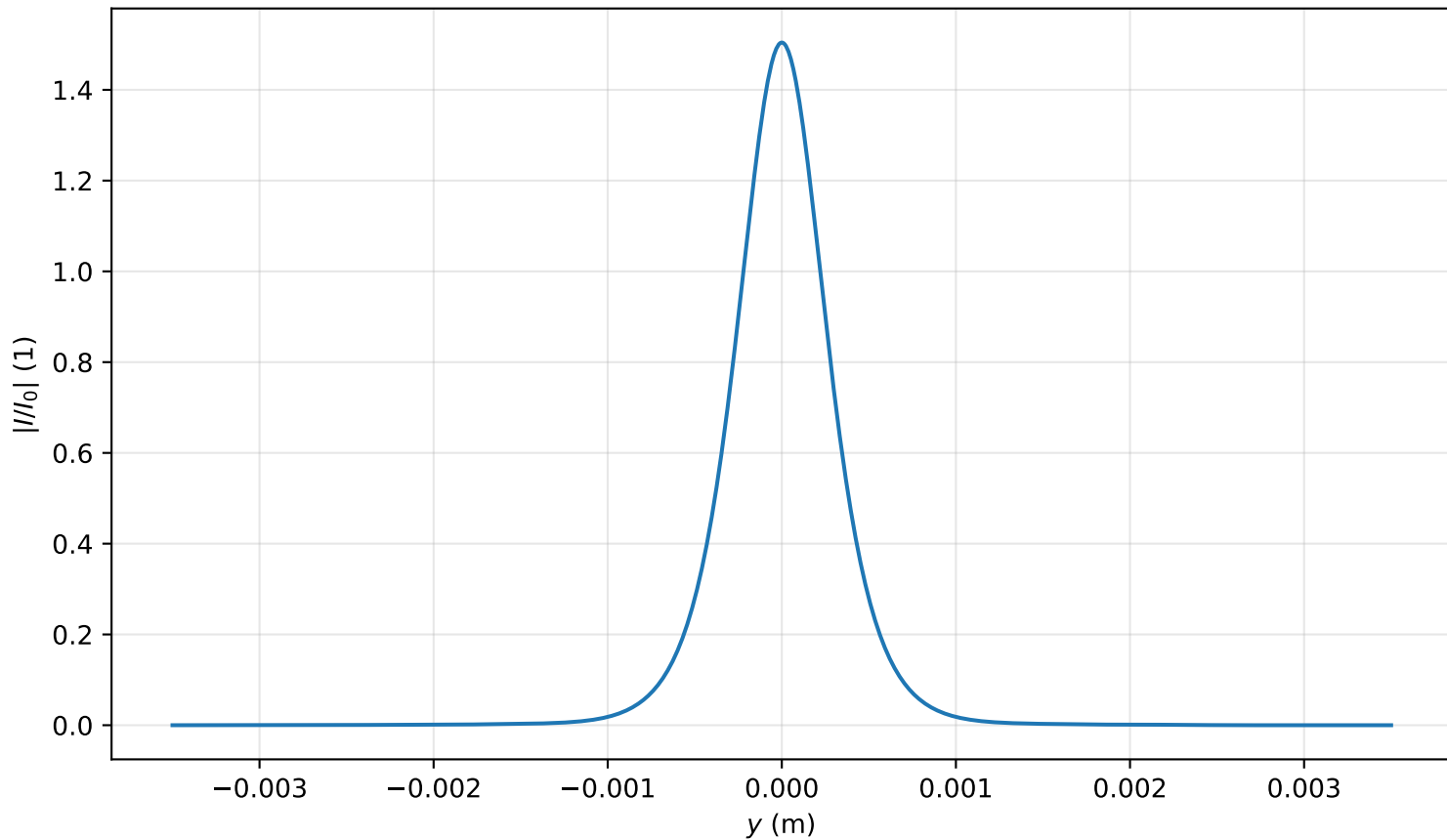
Intensity profile I(x=0, y, z=3.423)/I_0 , P_{in}=0.9P_{cr} , artificial time
